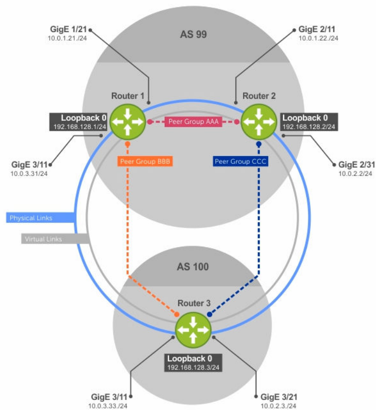
Figure 24. Sample Configurations
